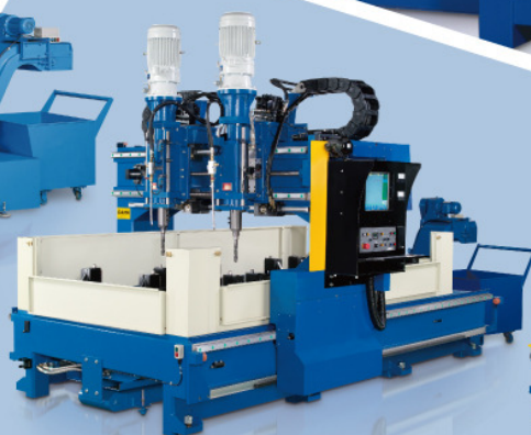
DMD-1224 / 1235 / 1635 / 1640 Joint Plate CNC Two Spindles Drilling Machine 數控雙主軸平板鑽孔機
