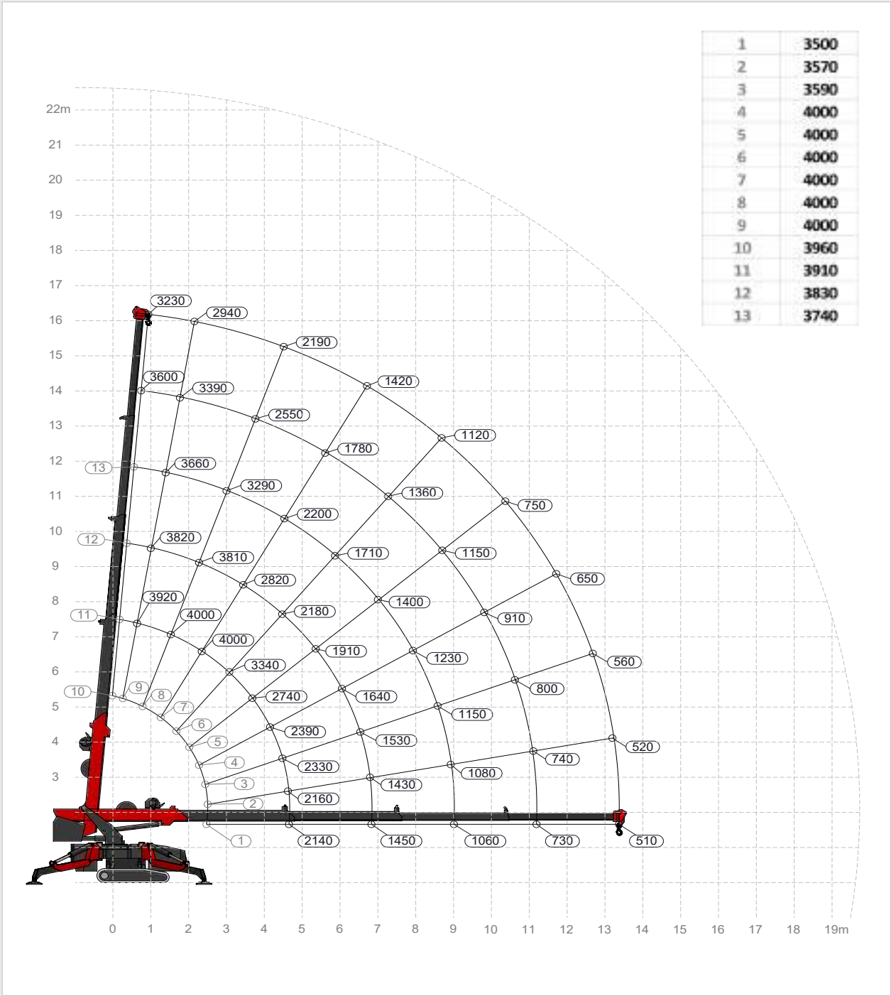
Main boom
