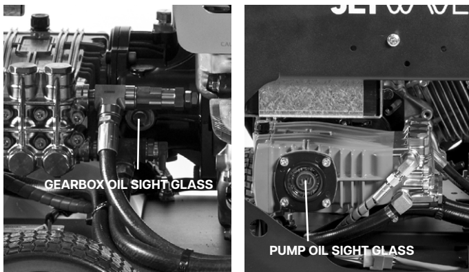
Figure.8 - Checking Pump and Gearbox Oil Level
