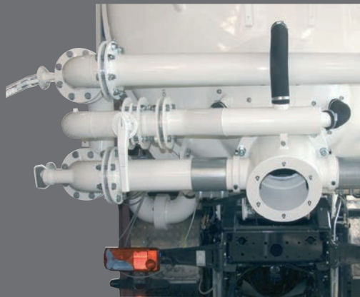
Pressure discharge device For flowing bulk material e.g. roof gravel.
