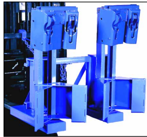
Model 288-2-2H for 1 or 2 drums. Two heads per drum.
